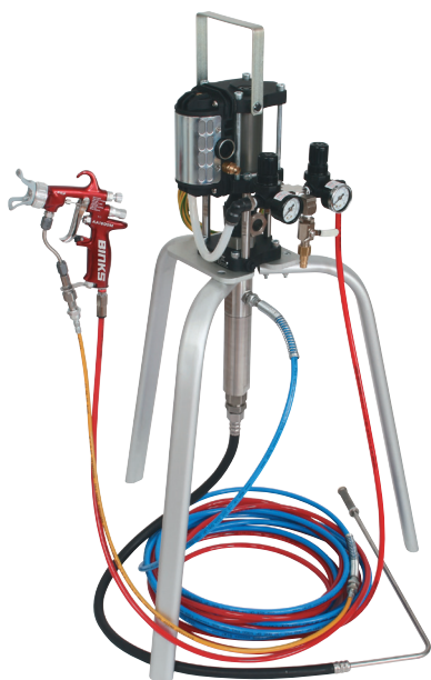
MX Lite Pump/Gun Outfit (Tripod-Mount)
